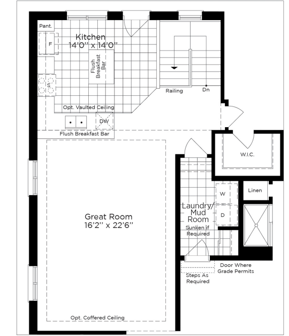
Opt. First Floor W/Alt. Kitchen Location
